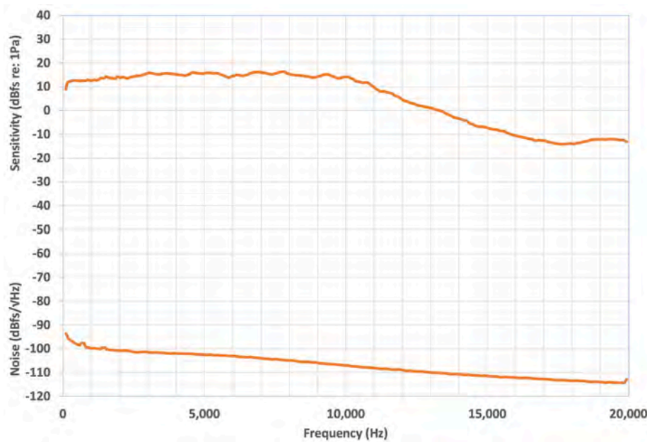
Figure 7. Sensitivity and Noise Floor, Linear Frequency Scale
