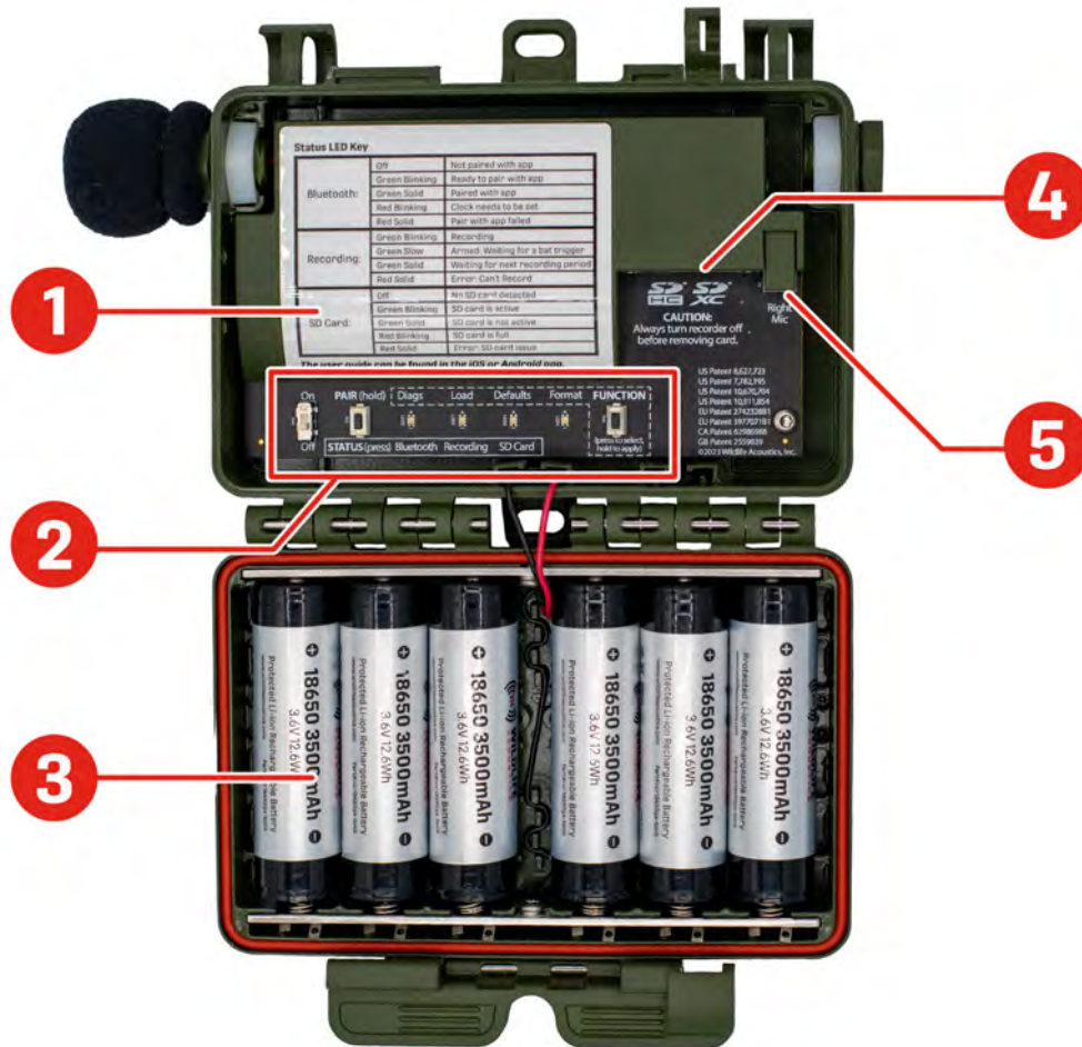
Figure 4. Internal Overview
